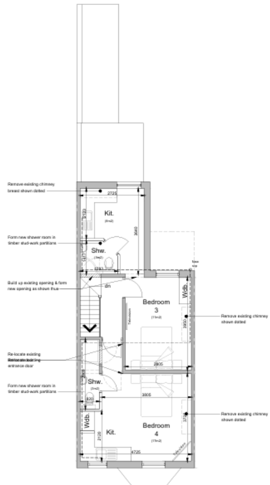
Proposed first floor plan Scale 1:50
