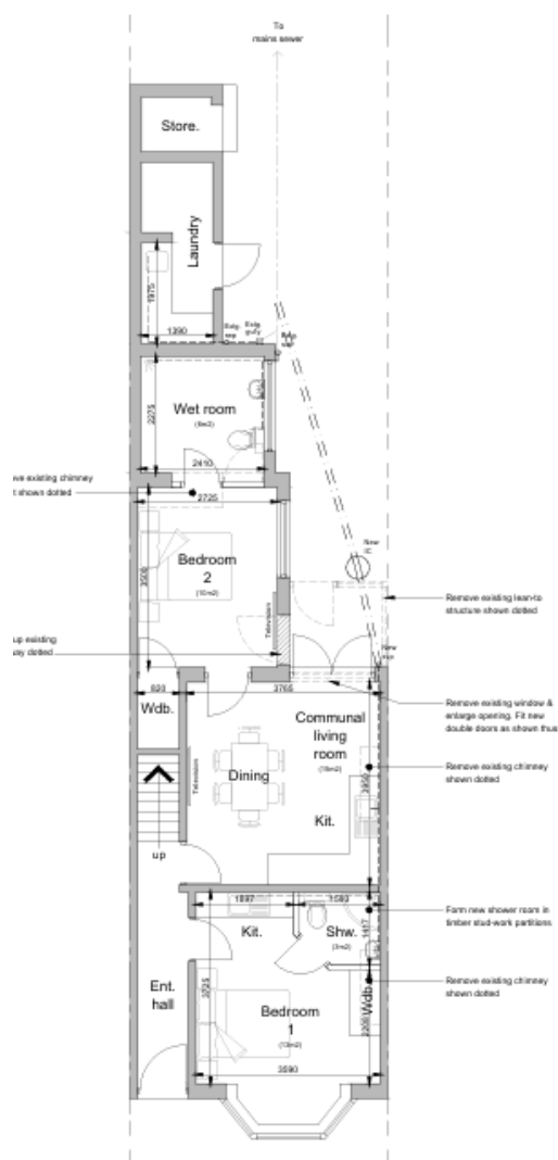
Proposed ground floor plan Scale 1:50
